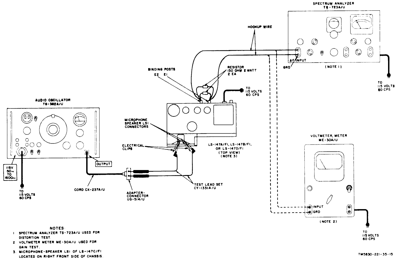
Figure 12. Distortion and gain test setup.
