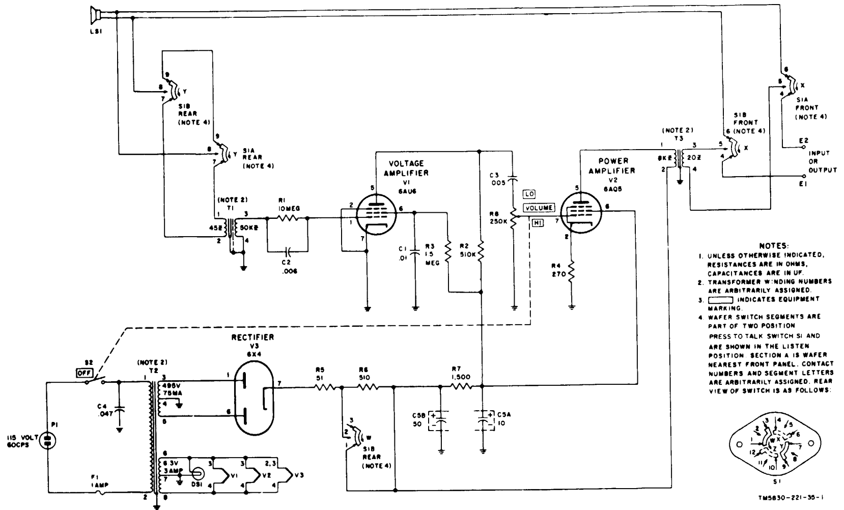
Figure 1. Intercommunication Station LS-147A/FI or LS-147B/FI, schematic diagram.
